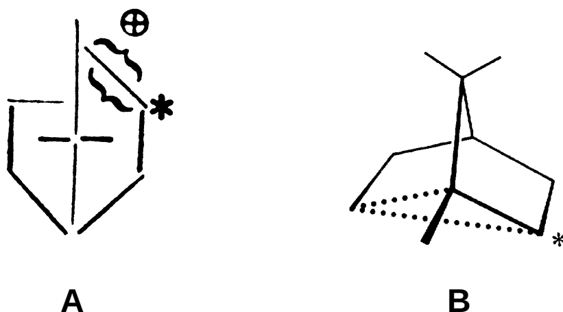
FIGURE 1. TWO DIFFERENT REPRESENTATIONS FOR THE ISOBORNYL CATION: (A) AS FIRST REPORTED IN 1939 AND (B) AS REDRAWN IN 1965. PERMISSION TO REPRINT (A) GRANTED BY THE ROYAL SOCIETY OF CHEMISTRY, CAMBRIDGE CB4 4WF, UK; PERMISSION TO REPRINT (B) GRACIOUSLY GRANTED BY THE PUBLISHER [16].
